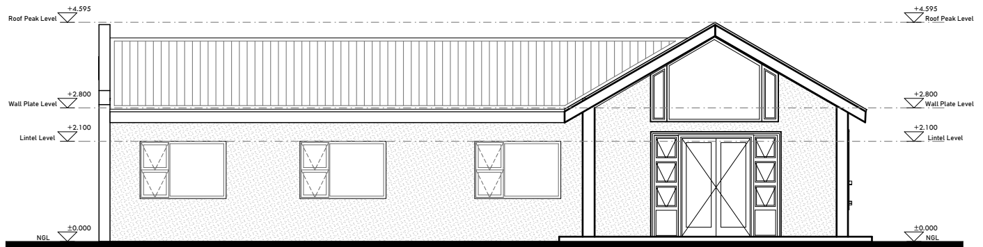
BACK
