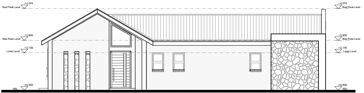
FRONT
