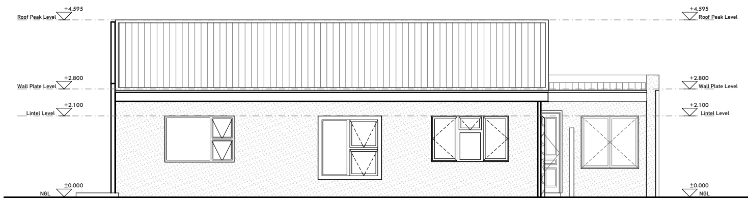
SIDE
